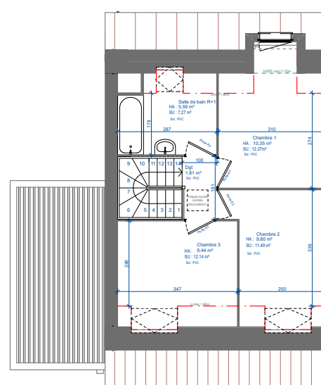
R+ Comble
