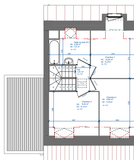
R+ Comble
