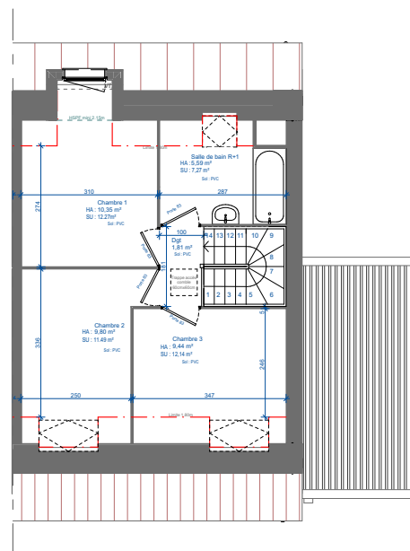
R+ Comble
