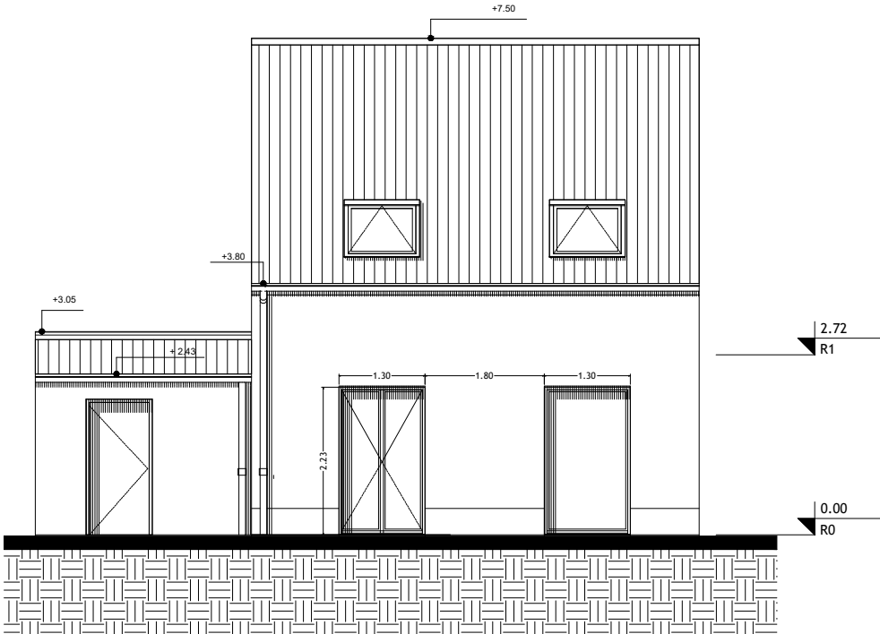
FAÇADE ARRIERE
